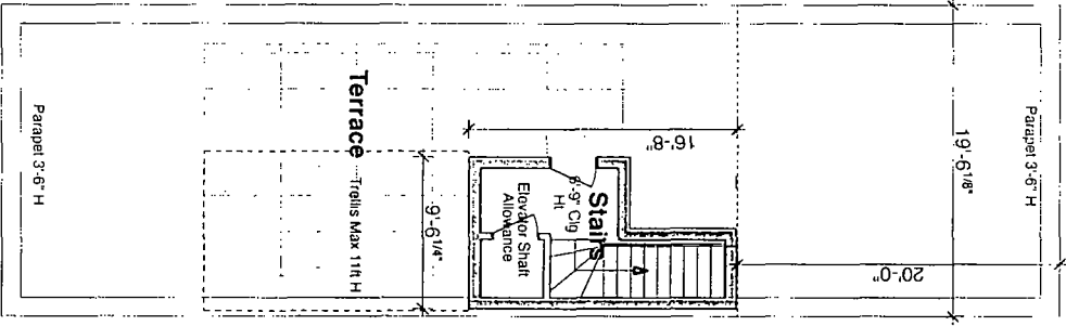
3rd Floor Plan
