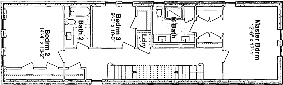
2nd Floor Plan
