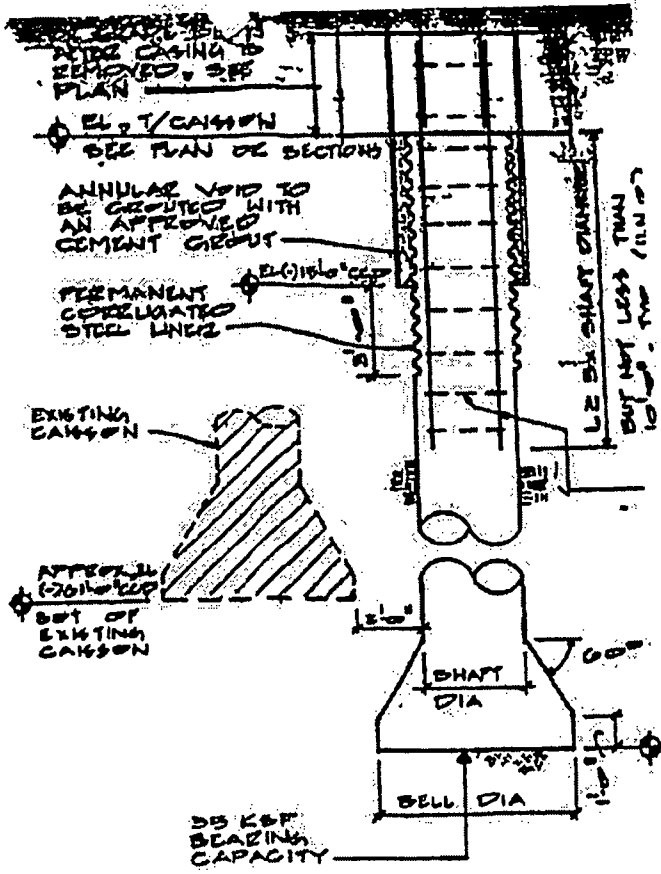
2 TYPICAL CAISSON DE NO SCALE
