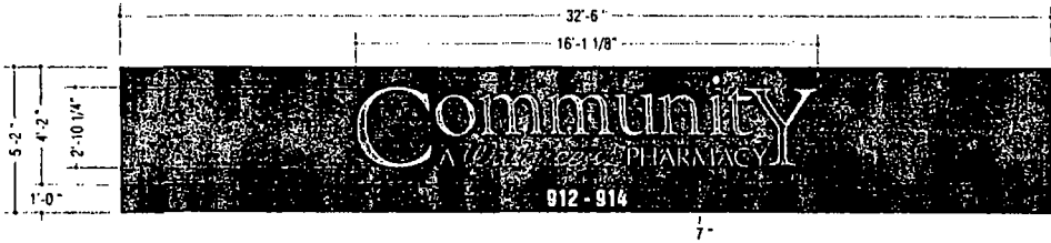
NEW AWNING LAYOUT/DIMENSIONS 1/4" = 1'-0"
