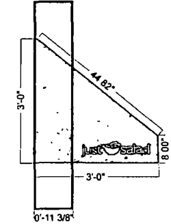
Building Column
