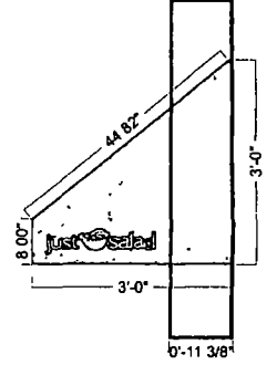
Building Column
