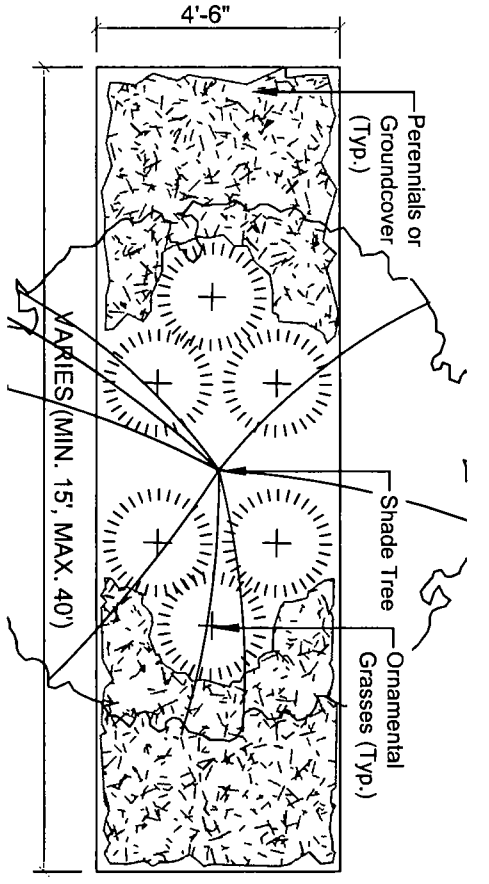
1 PLANTER - TYPICAL PLAN NTS
