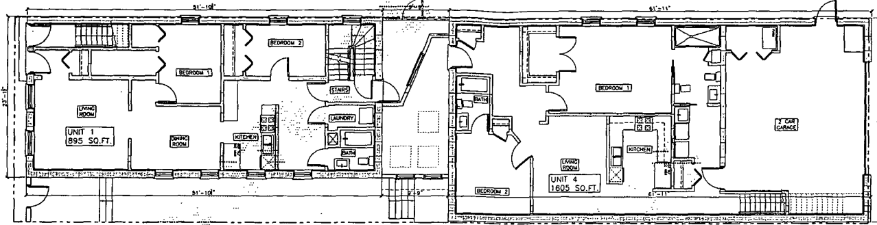
⊕ EXIST. FIRST FLOOR PLAN
