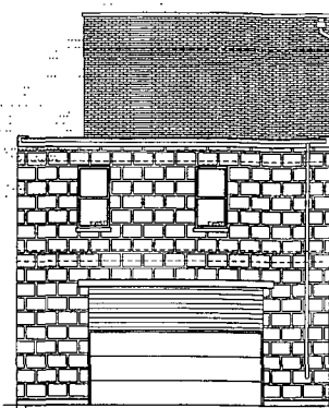
EXIST. EAST ELEVATION SCALE 3/16" = 1'-0"
