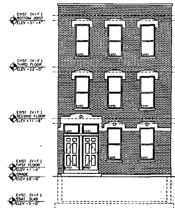
EXIST. WEST ELEVATION SCALE 3/16" = 1'-0"
