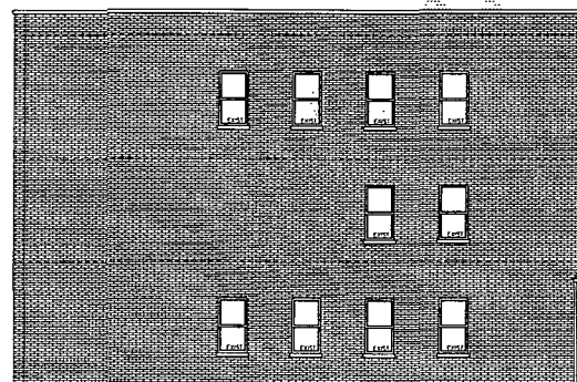
EXIST. SOUTH ELEVATION SCALE 3/16" = 1'-0"
