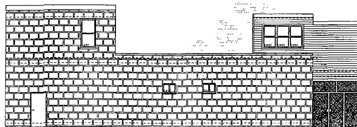
EXIST. NORTH ELEVATION SCALE 3/16" = 1'-0"
