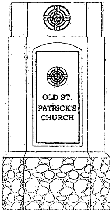
1 Elevation- Street 3'-4" x 1'-0"
