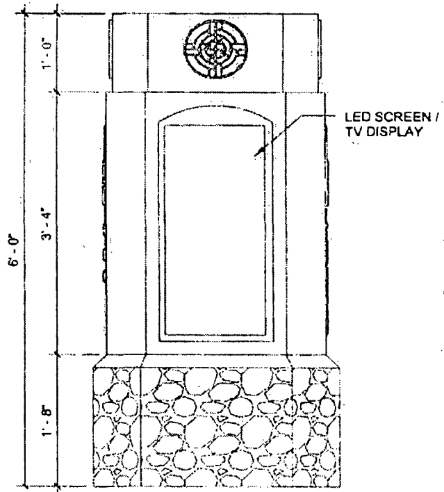
2 Elevation- Sidewalk 3'-4" x 1'-0"
