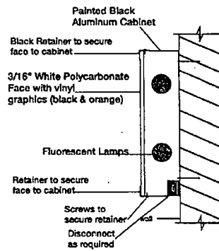
Side Elevation - No Scale
