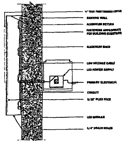
Standard Form 412 Light Box with Push Through Acrylic Lettering - LED Backlight
