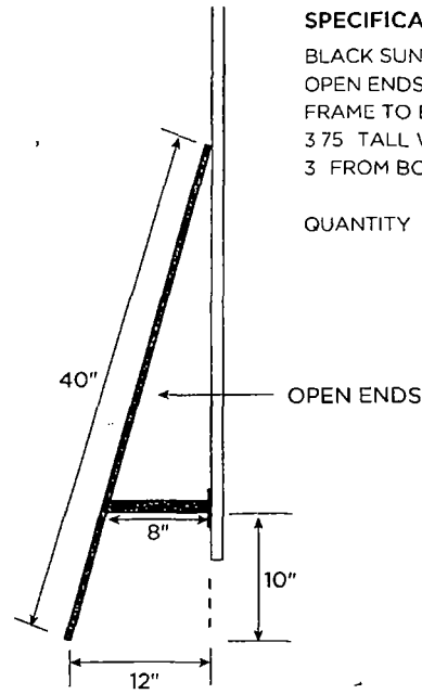
SIDE DETAIL
