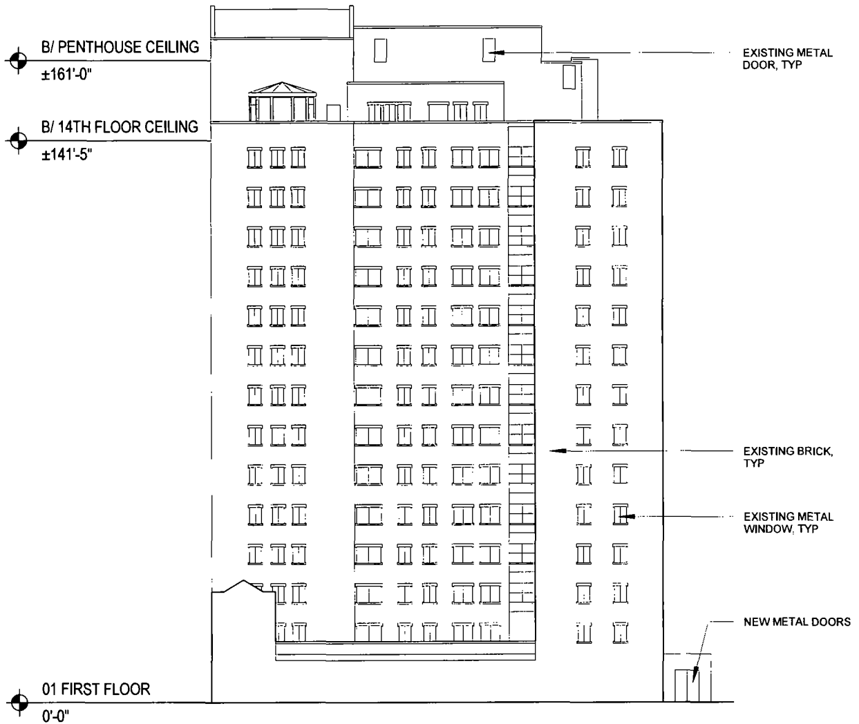
WEST ELEVATION
