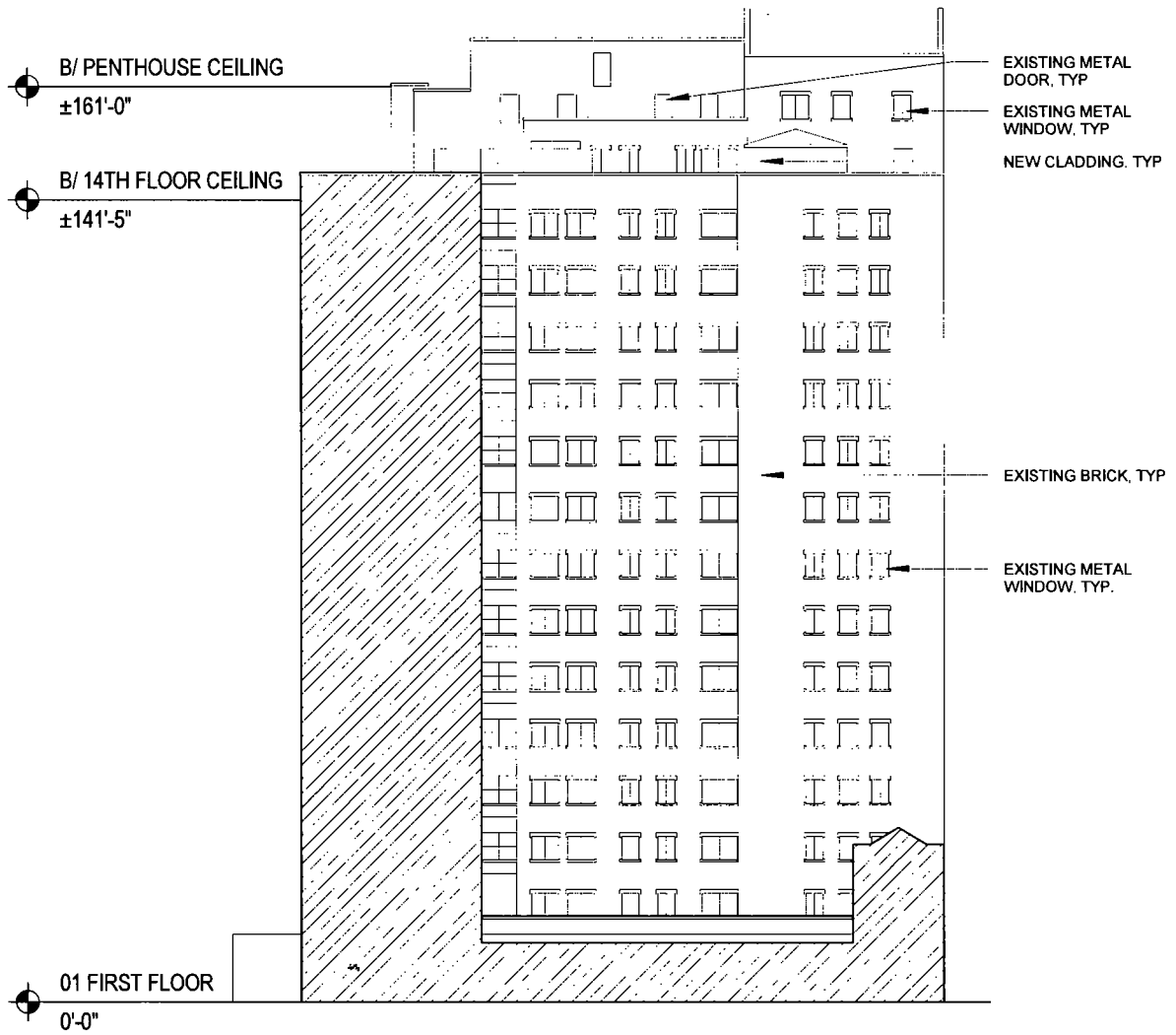
EAST ELEVATION
