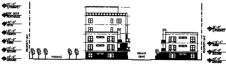
ARGYLE STREET ELEVATION
