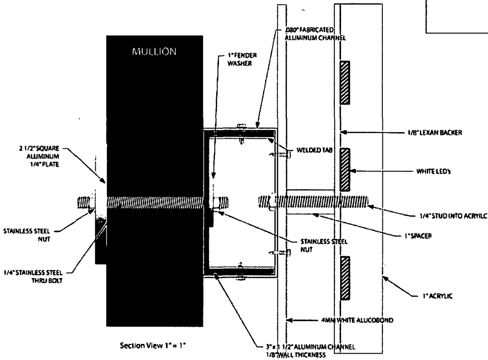
Section View 1/8" = 1"
