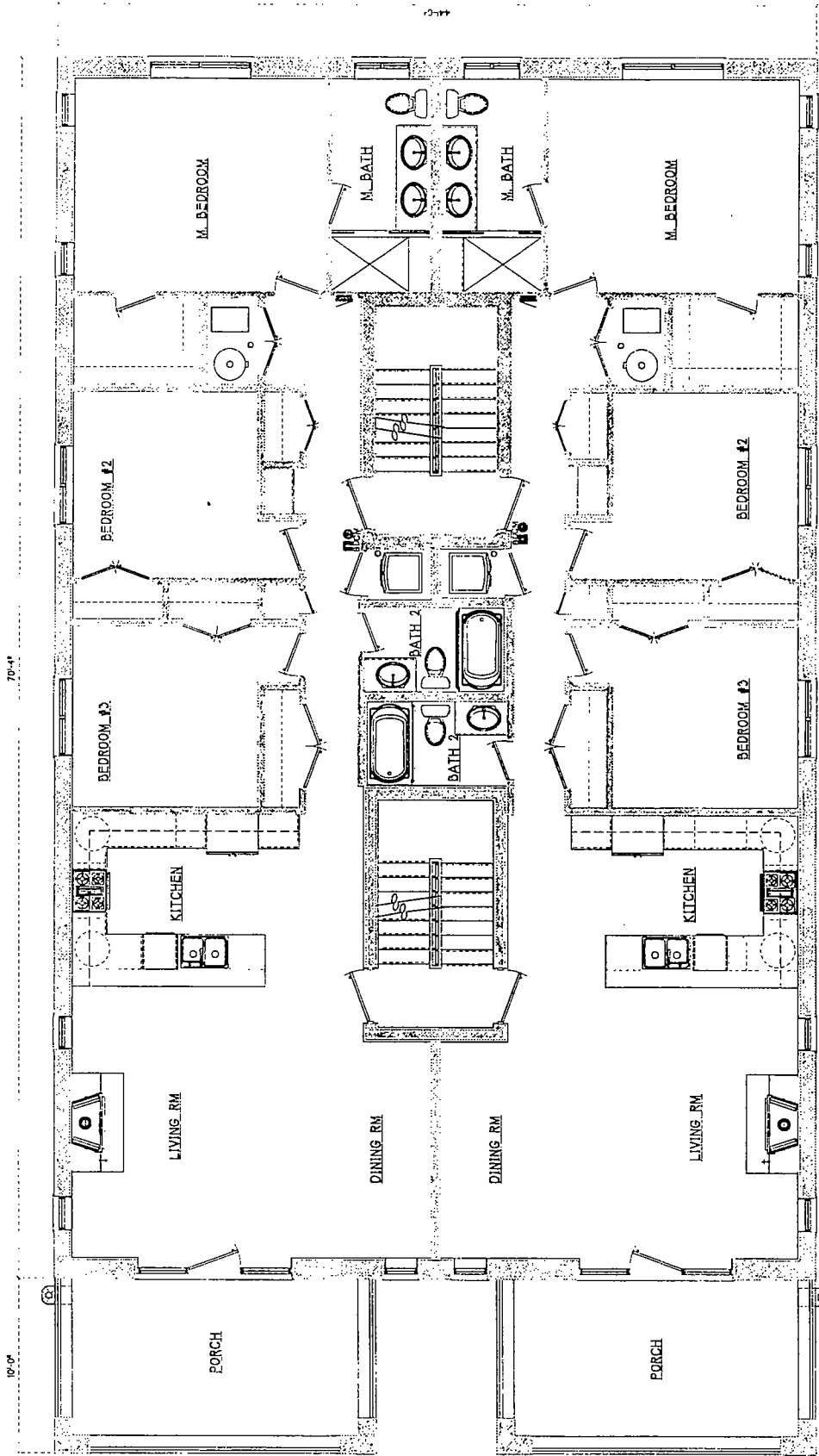
FOURTH FLOOR PLAN
