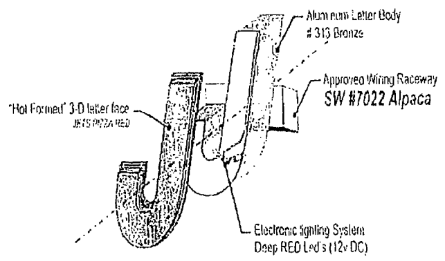
Exploded View
