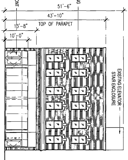
NORTH ELEVATION 1/8" = 1'-0"
