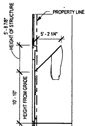
② TYPICAL FLAGPOLE SECTION 1/8" = 1'-0"
