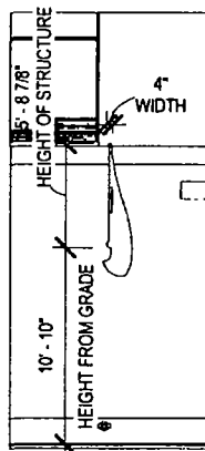
① TYPICAL FLAGPOLE ELEVATION 1/8" = 1'-0"
