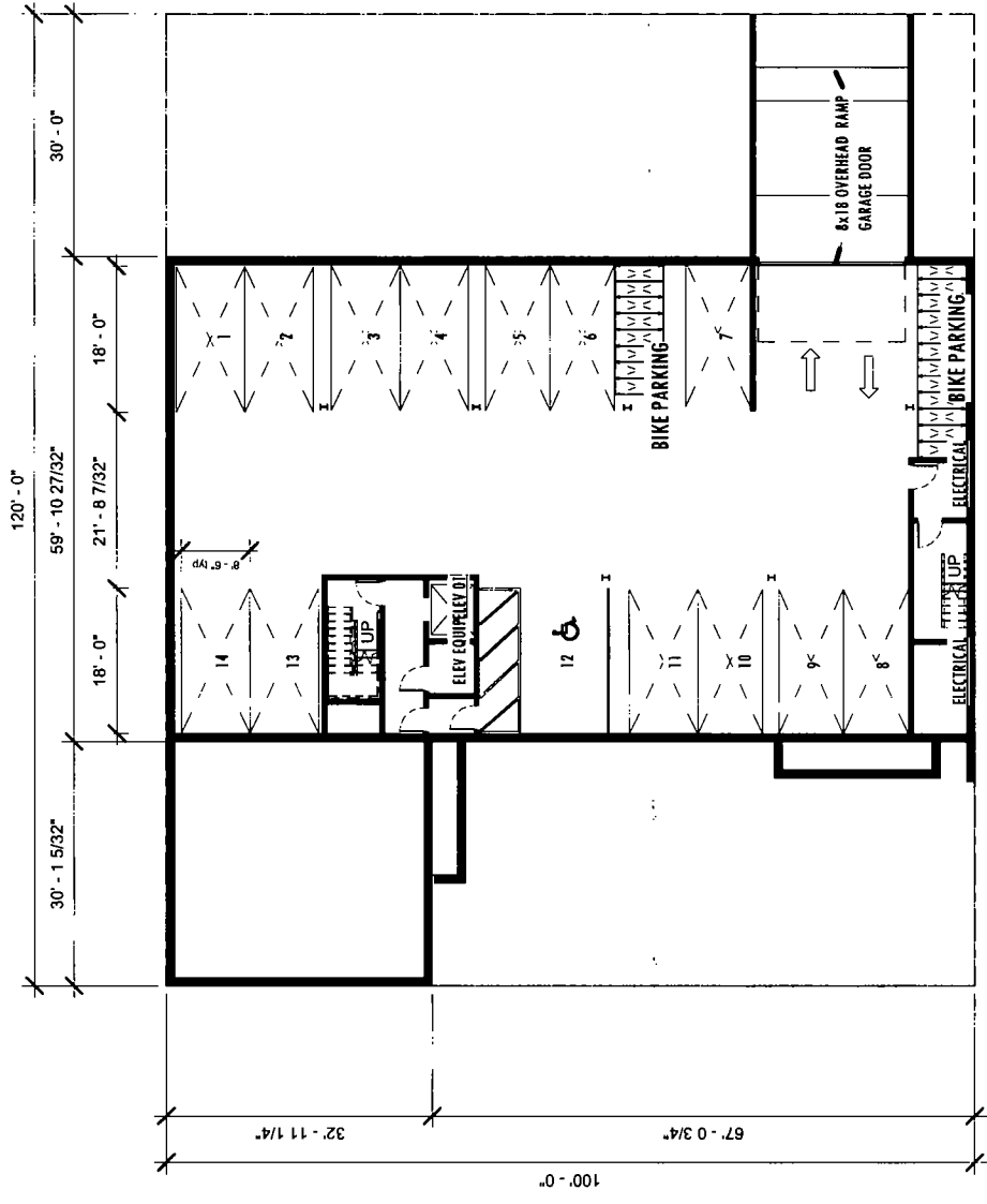
1 Basement CGM 1/16" = 1'-0"
