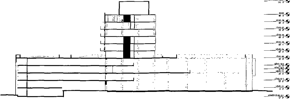
BUILDING SECTION 0' 40'
