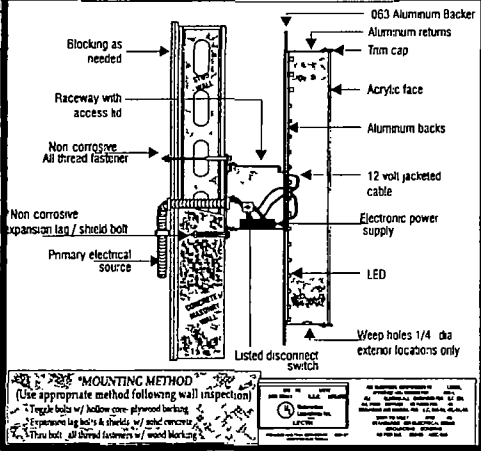
LED CHANNEL - RACEWAY MOUNT
