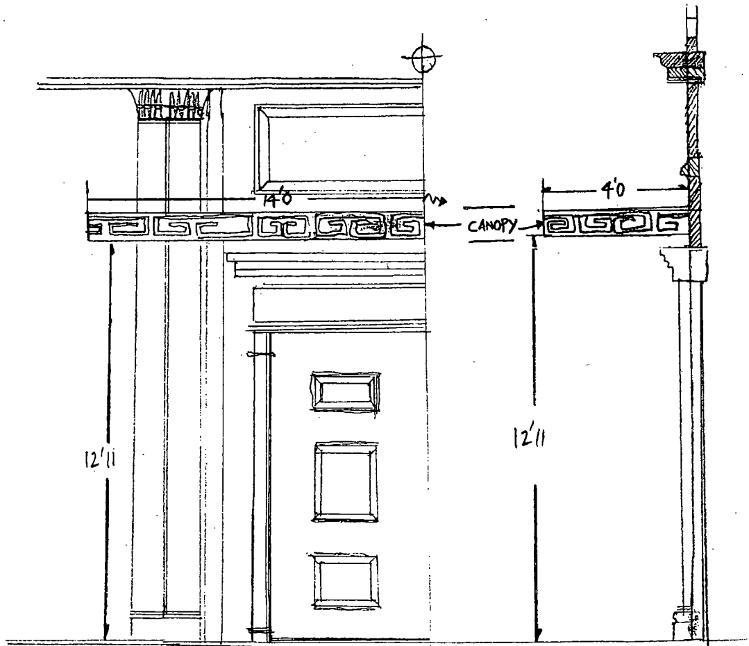
HALF ELEVATION OF NORTH ENTRANCE SECTION DEVON AVENUE
