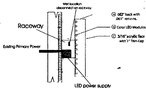
Typical Raceway Mount channel Letters with LED's
