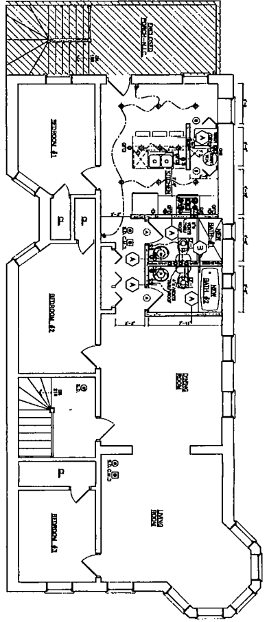
PROPOSED THIRD FLOOR PLAN DATE: 1/27/2007
