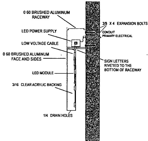
BACK LIT CHANNEL LETTER SIGN LED ILLUMINATED W/RACEWAY
