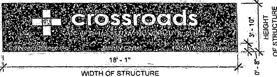
② FRONT ELEVATION- AWNING 1/4" = 1'-0"
