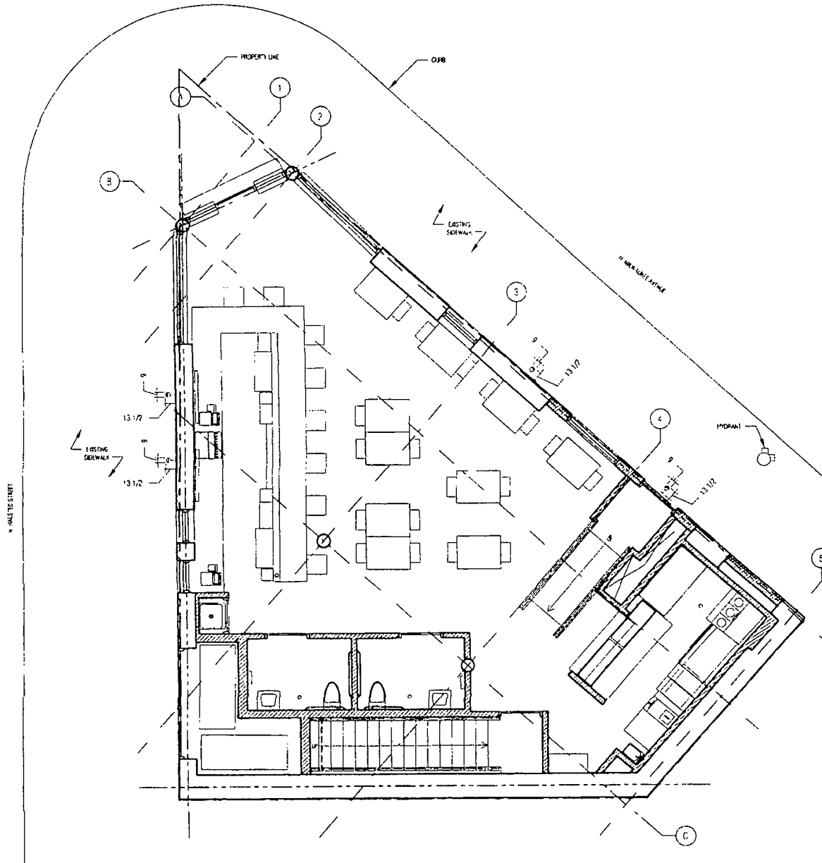
01 Maillard First Floor Plan 1/8" = 1'-0"
