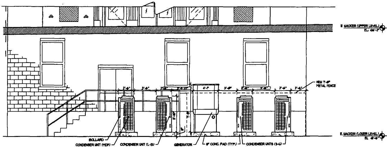
1 GENERATOR & CONDENSER UNIT LOCATION ELEVATION SCALE: 1/4" = 1'-0"
