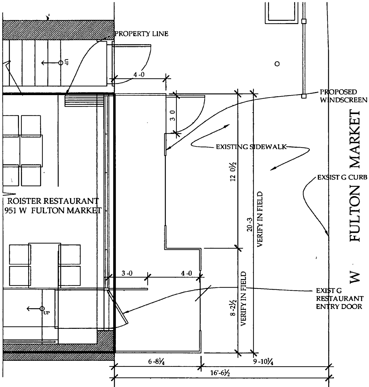
PLAN SCALE 1/4" = 1'-0"
