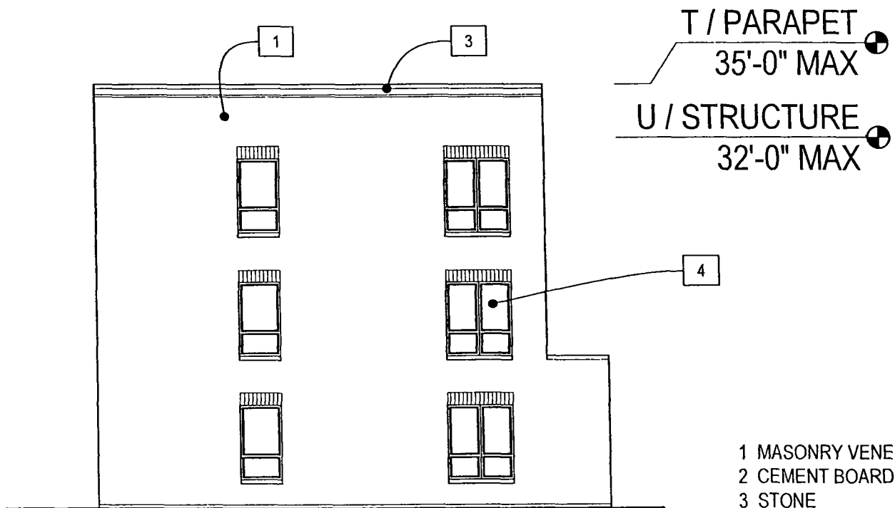
TYPE G - FRONT ELEVATION
