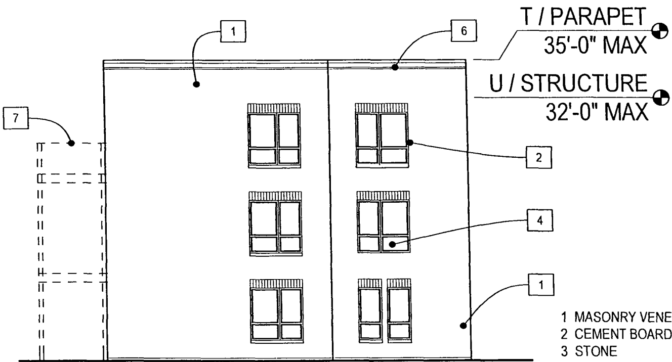
TYPE G - SIDE ELEVATION
