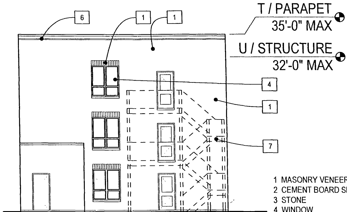
TYPE A - REAR ELEVATION
