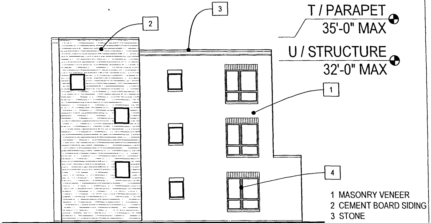
TYPE H - SIDE ELEVATION
