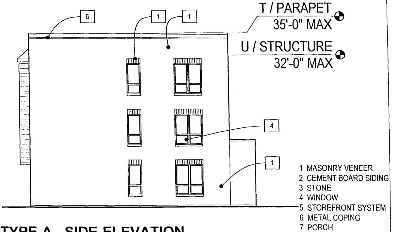
TYPE A - SIDE ELEVATION
