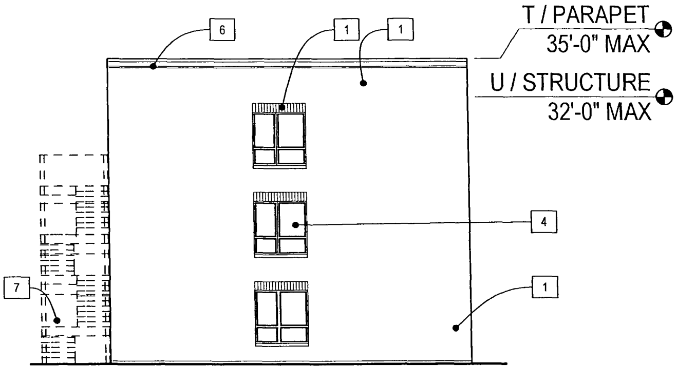
TYPE A - SIDE ELEVATION
