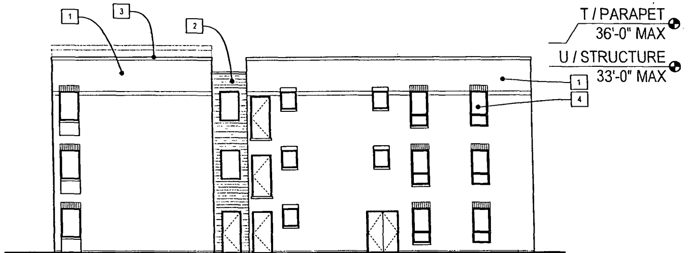
TYPE J - REAR ELEVATION
