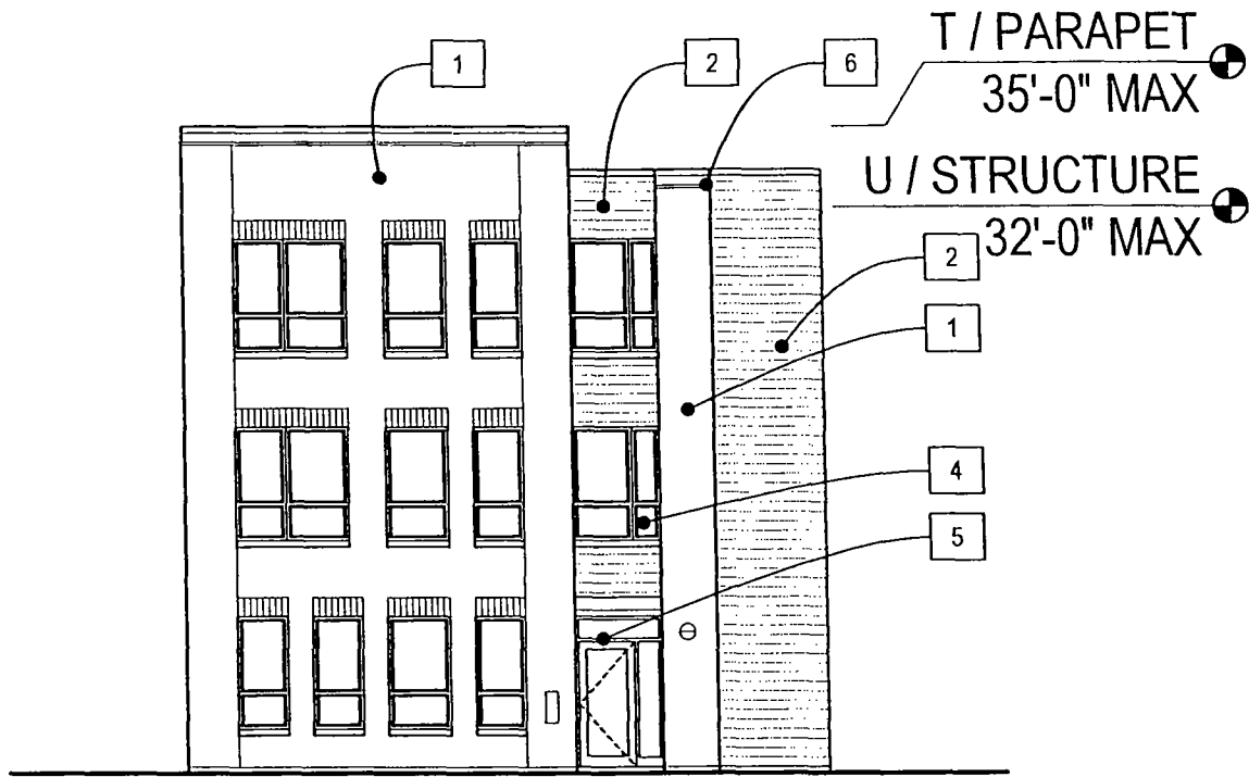
TYPE H - FRONT ELEVATION
