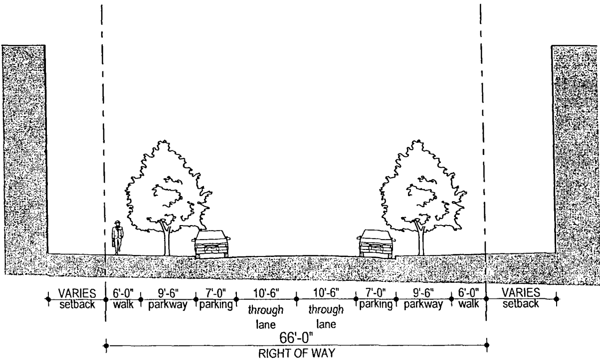
S MILLARD AVE - 66' ROW
