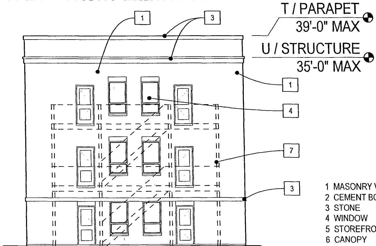
TYPE D - FRONT ELEVATION
