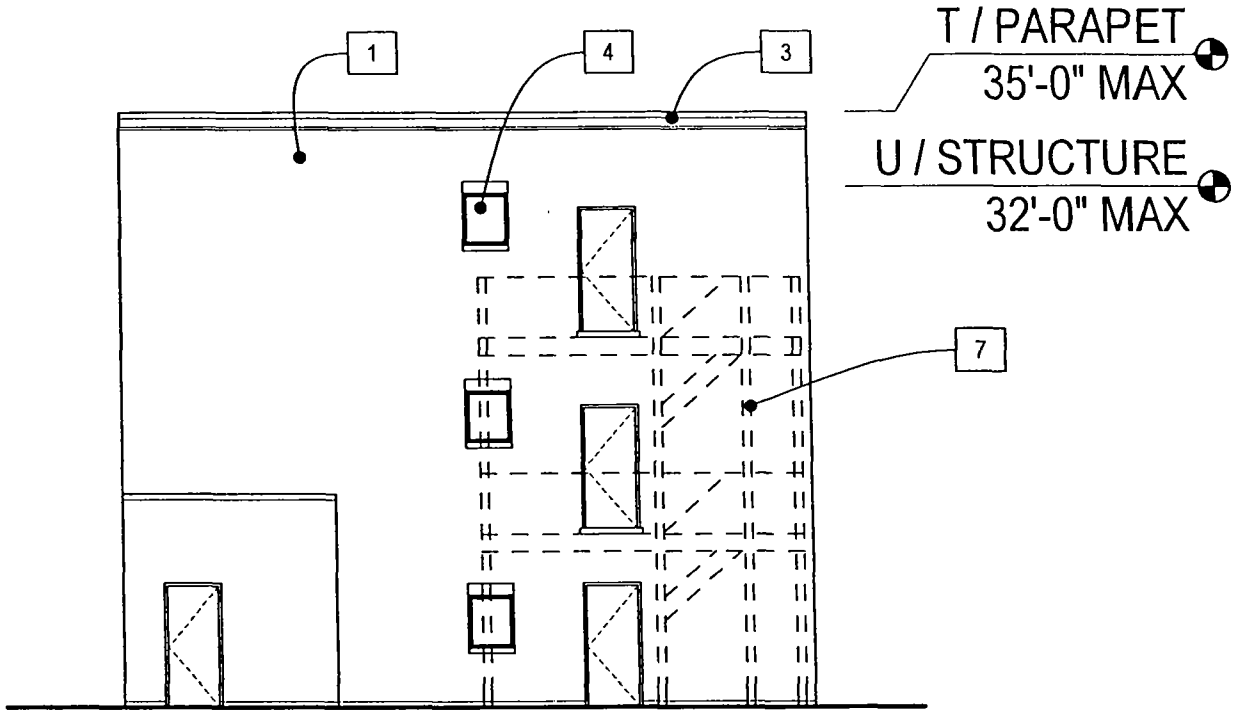
TYPE G - REAR ELEVATION
