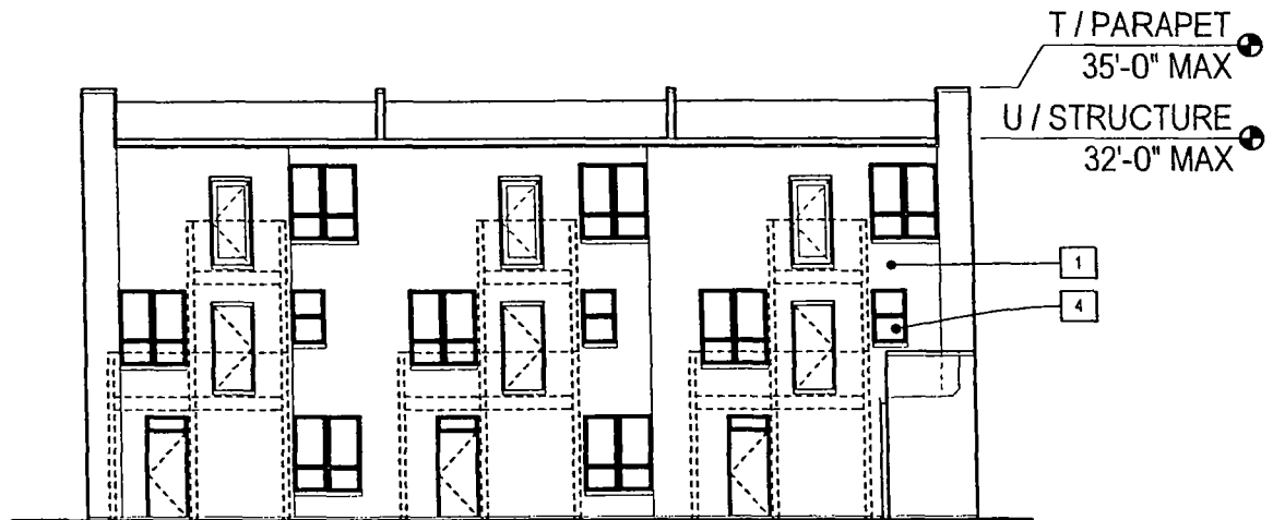
TYPE C - REAR ELEVATION
