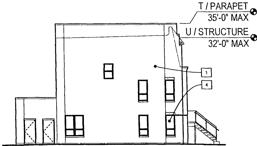
TYPE C - SIDE ELEVATION
