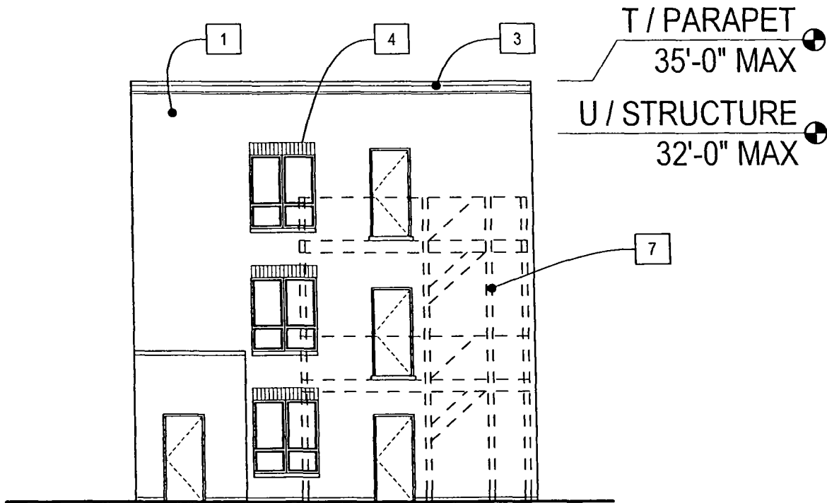
TYPE H - REAR ELEVATION
