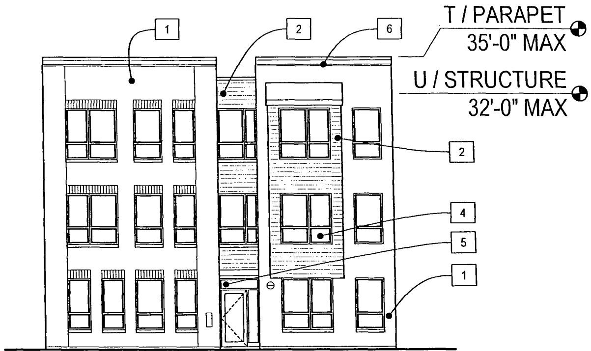
TYPE G - FRONT ELEVATION
