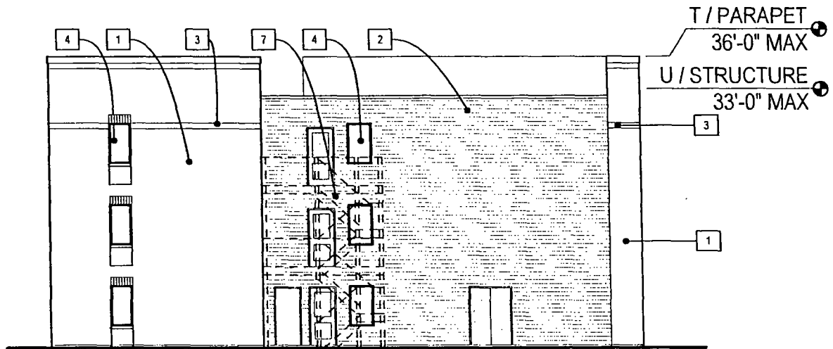
TYPE B - REAR ELEVATION
