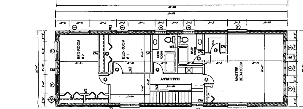
2ND FLR PLAN SCALE: 1/8" = 1'-0"
