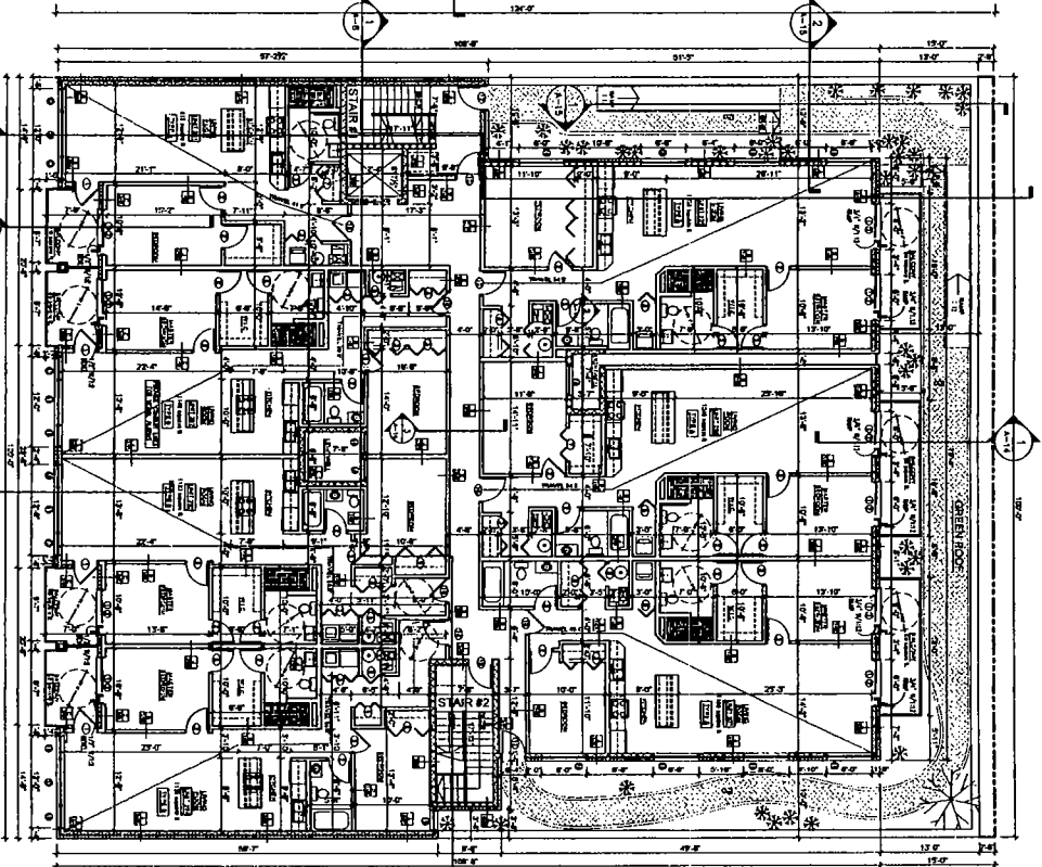
2 SECOND FLOOR PLAN
