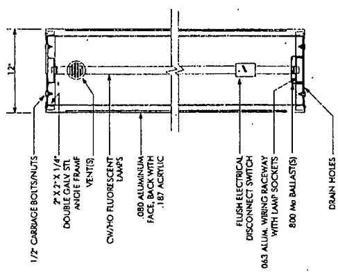
DOUBLE FACED INTERNALLY ILLUMINATED CABINET
