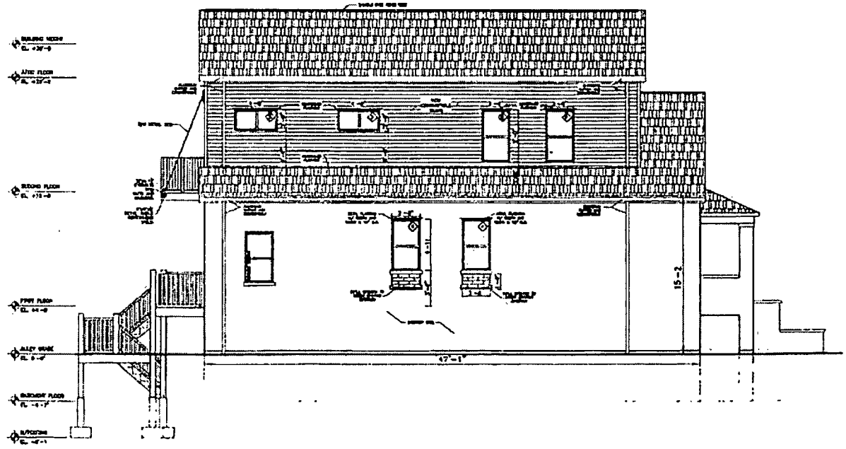
NORTH ELEVATION
