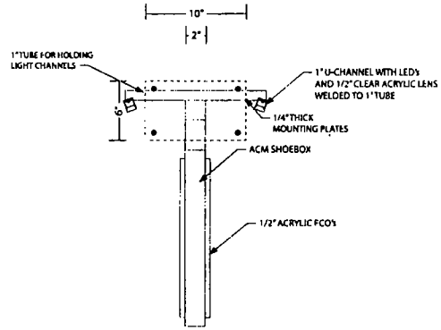
End View 1 1/2" = 1'-0"
