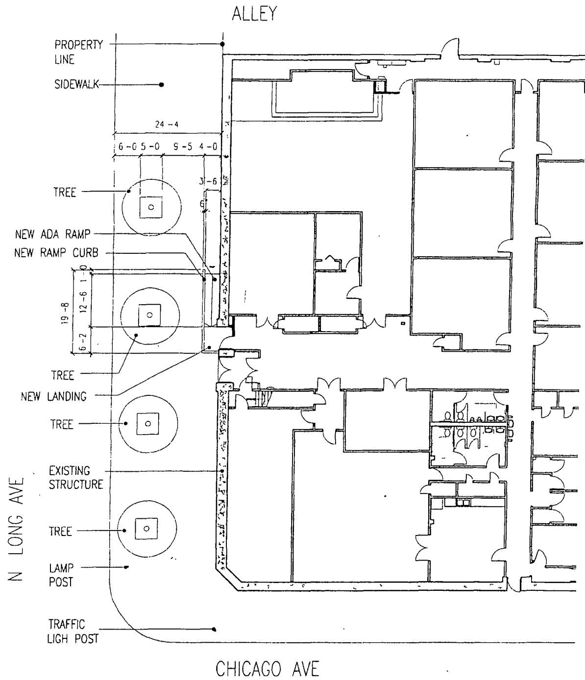
SITE PLAN 1" = 20' 0"
