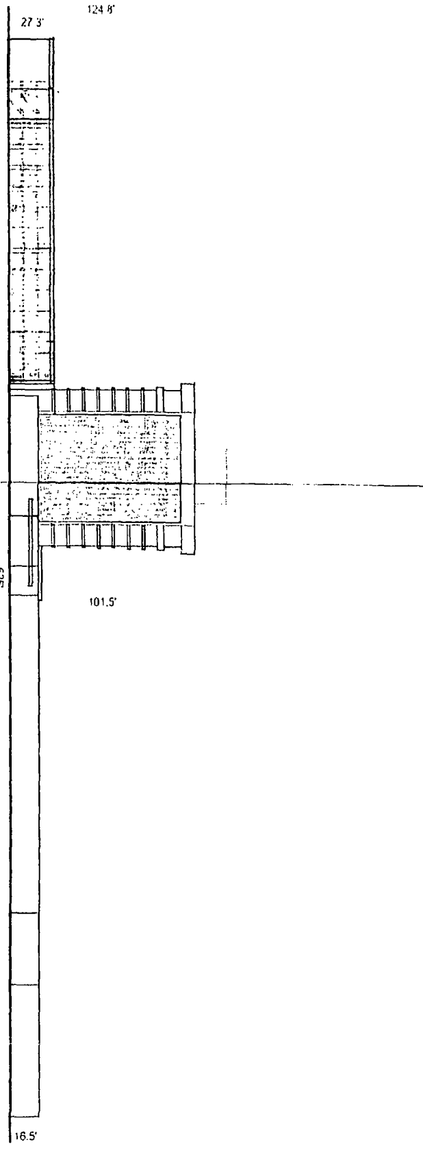
SOUTH ELEVATION
