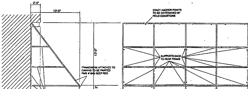
FRONT FRAME DETAIL 3/16" = 1'-0"
