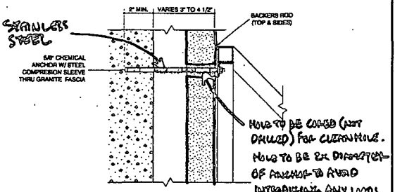
CANOPY MOUNTING DETAIL 1/2" = 1'-0"
