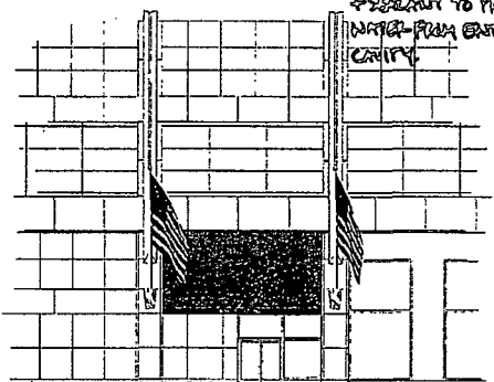
PARTIAL NORTH ELEVATION / CANOPY LOCATION 1/16" = 1'-0"
