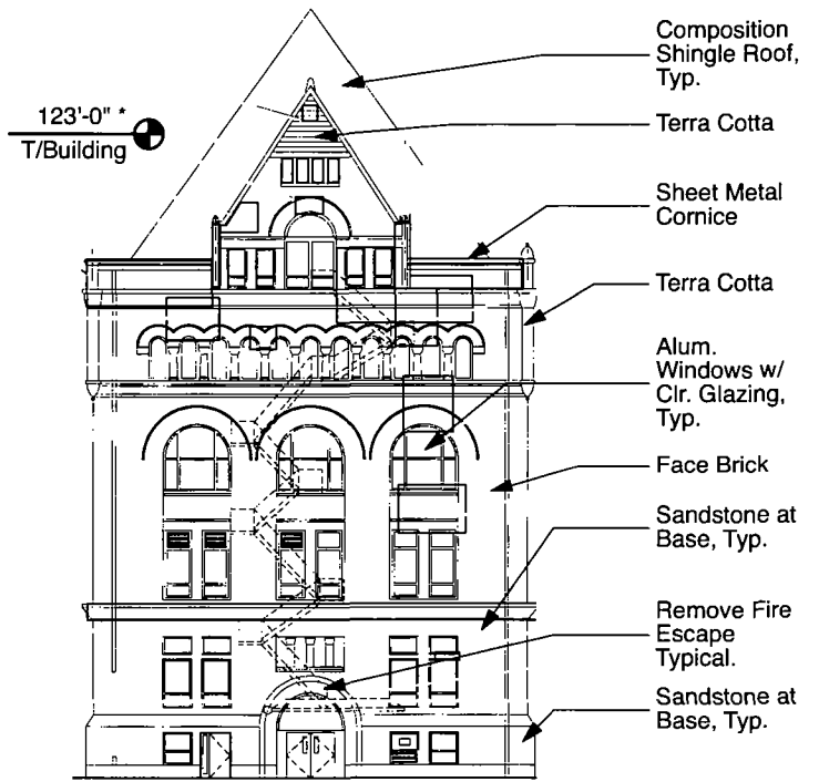
North Elevation - Main Building
