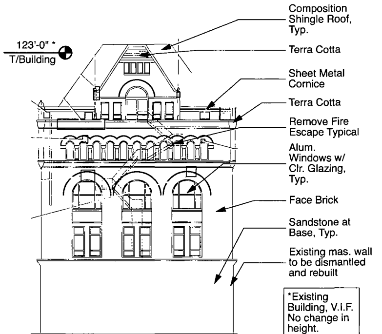
South Elevation - Main Building
