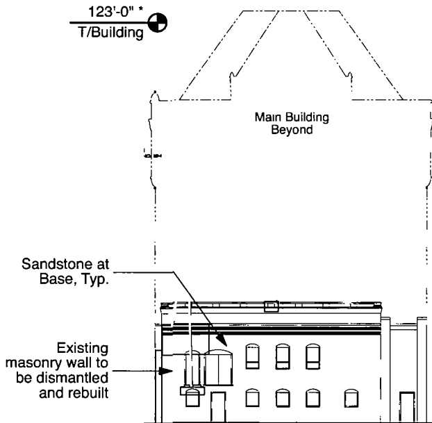
South Boiler House Elevation
