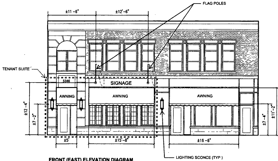
FRONT (EAST) ELEVATION DIAGRAM SCALE 1/8" = 1'-0"
