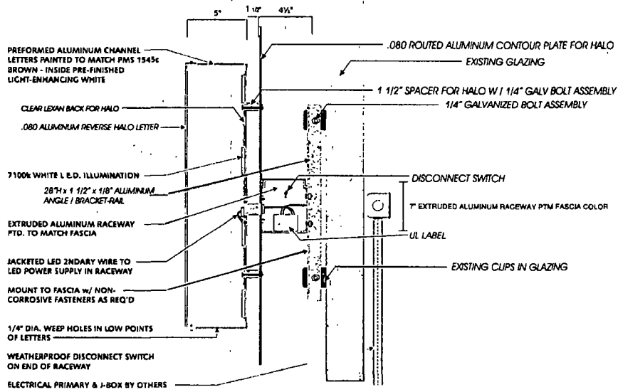
Typical Detail - HALO ILLUMINATED CHANNEL LETTERS WITH CONTOUR PLATE
