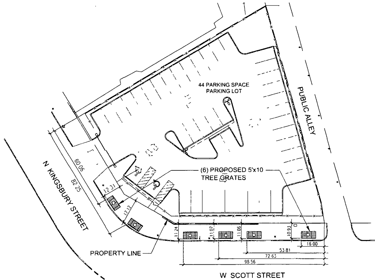
TREE GRATE LOCATION PLAN SCALE 1" = 30'-0"
