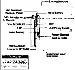
SIDE VIEW- Front Lit Channel Letter on Raceway
