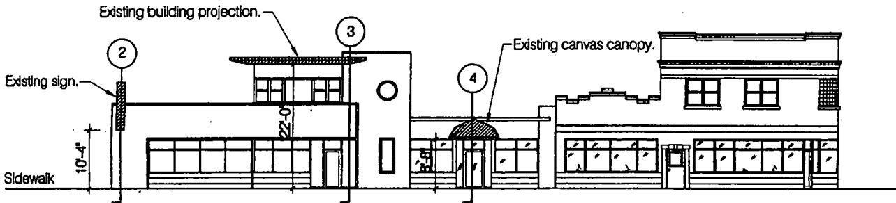
1 North Elevation Scale: 1/16" = 1'-0"
