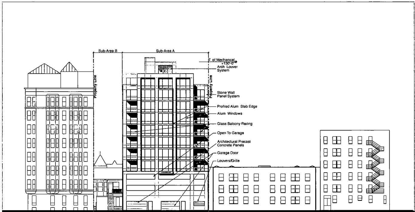
North Elevation
