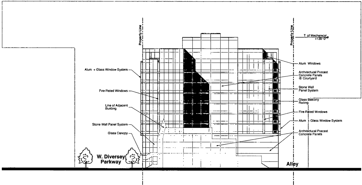
East Elevation
