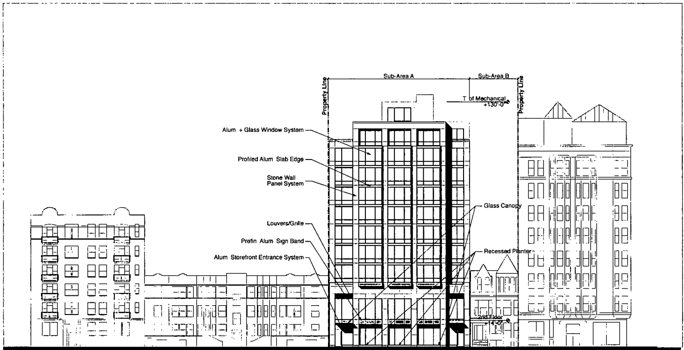
South Elevation
