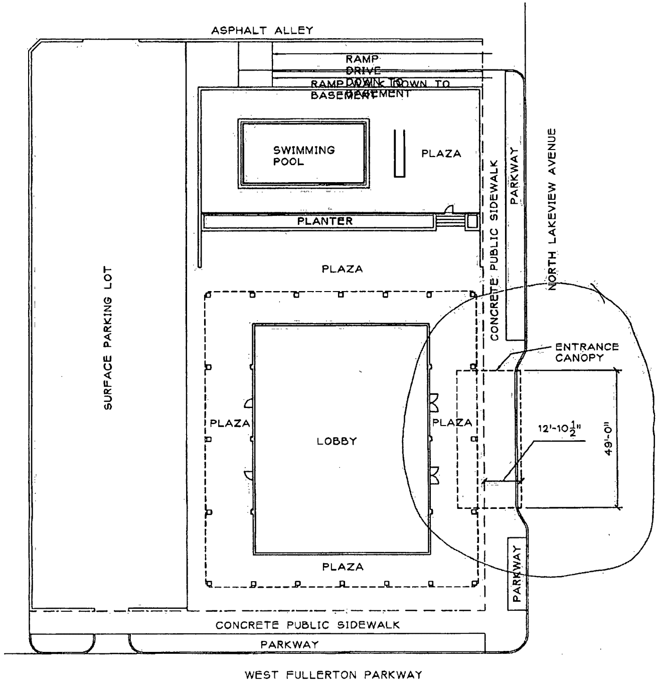
1 SITE PLAN SCALE 1" = 30'
