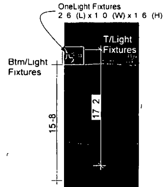
5 Light Fixture 1558 N Washtenaw Ave NOT TO SCALE
