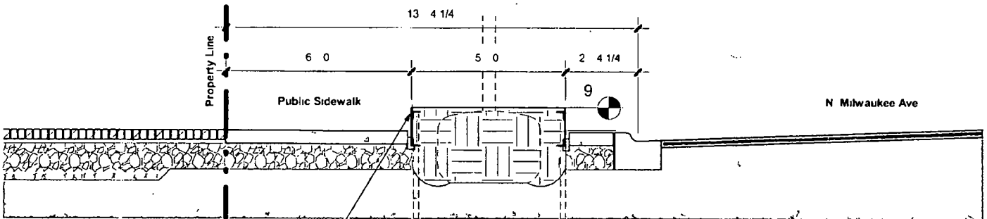
① Public Way Section - Planter 1/4" = 1'-0"
