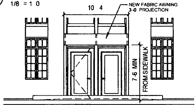
3 ELEVATION 1/8" = 1'-0"
