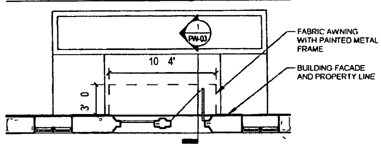
2 PARTIAL PLAN 1/8" = 1'-0"
