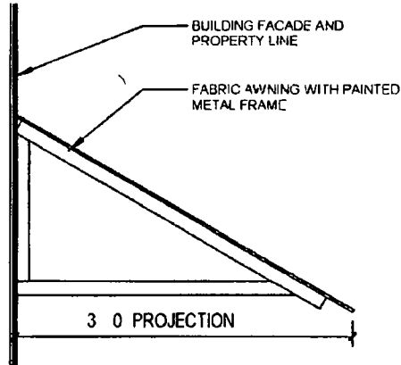
1 SECTION 3/4" = 1'-0"
