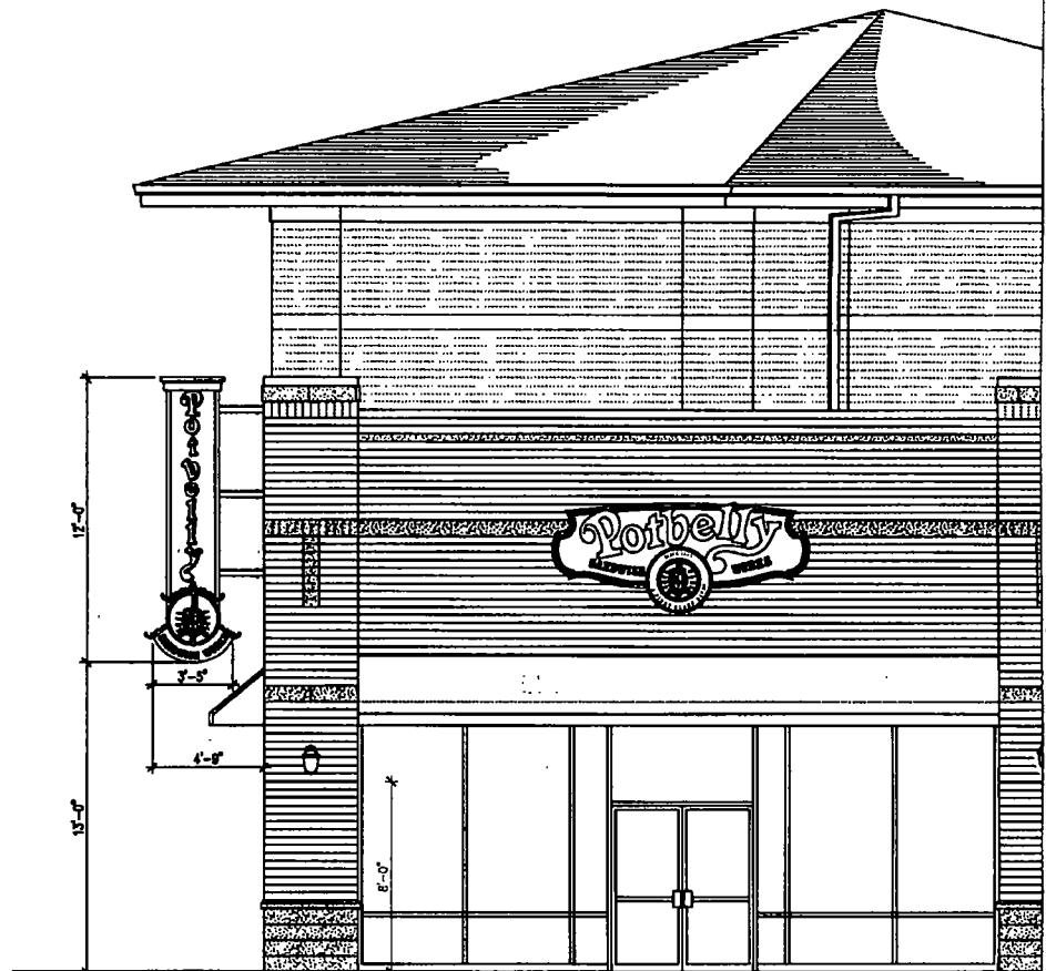
SOUTH ELEVATION SCALE 1/8" = 1'-0"
