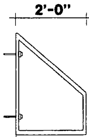
2' PROJECTION STEEL CLIPS WITH 3/8" EXPANSION BOLTS
